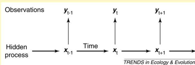
Figure 1. General structure of SSMs. The y_t are the data observed given the true, but unobserved, state \mathbf{x}_t . Horizontal arrows depict the process model prediction of the true state of the animal (Equation Ia) through time. Vertical arrows the observation model (Equation Ib).
